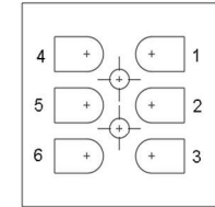
Screw terminals view
