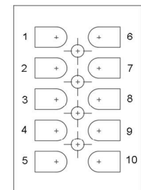
Screw terminal view
