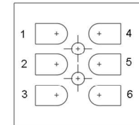
Screw terminal view
